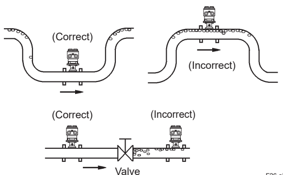
F26.ai Avoiding Air Bubbles
