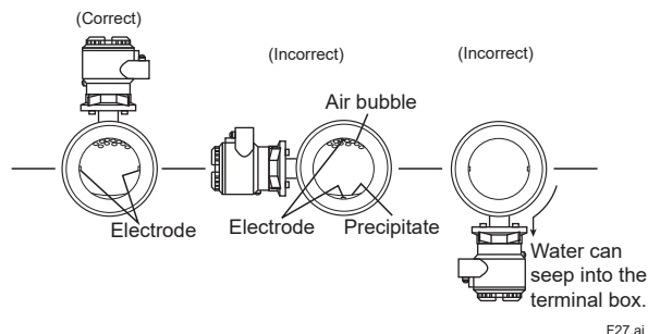
F27.ai Mounting Orientation
