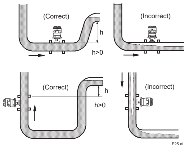
F25.ai Mounting Positions
